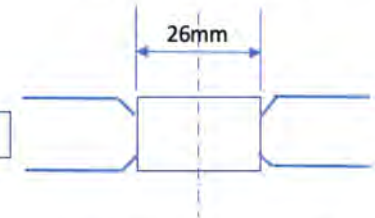
American / Japanese Tapered suits Double Nut
