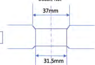
American / Japanese Tapered suits Double Nut
